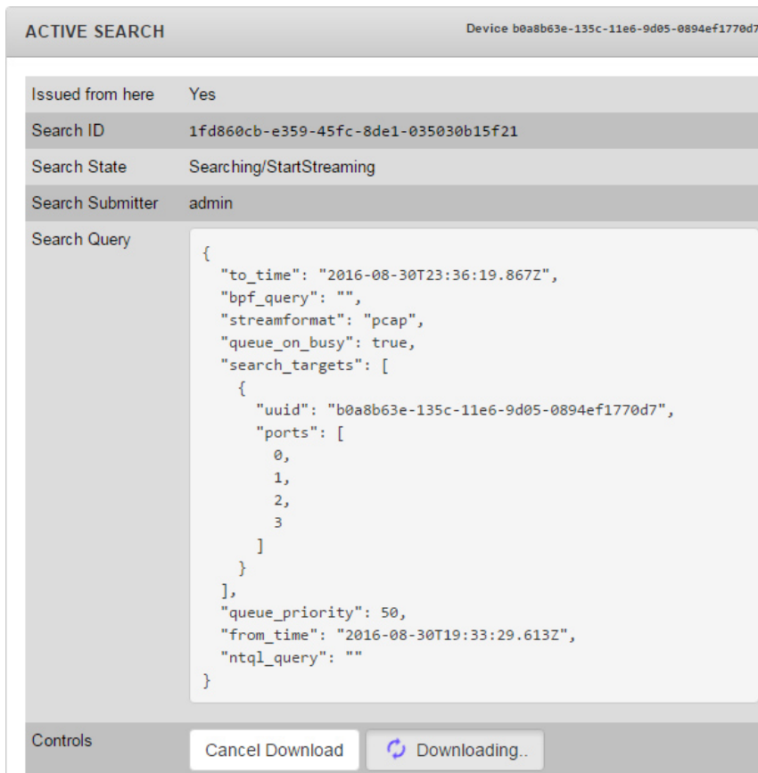
Figure 5. ACTIVE SEARCH widget
